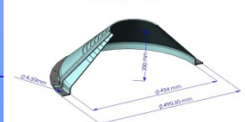
PIPETITE 7" to 14"
