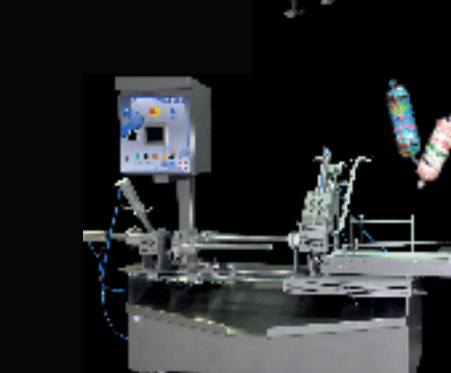
▲ FILL & CLIP automatic machine for ice cream "sausage"
