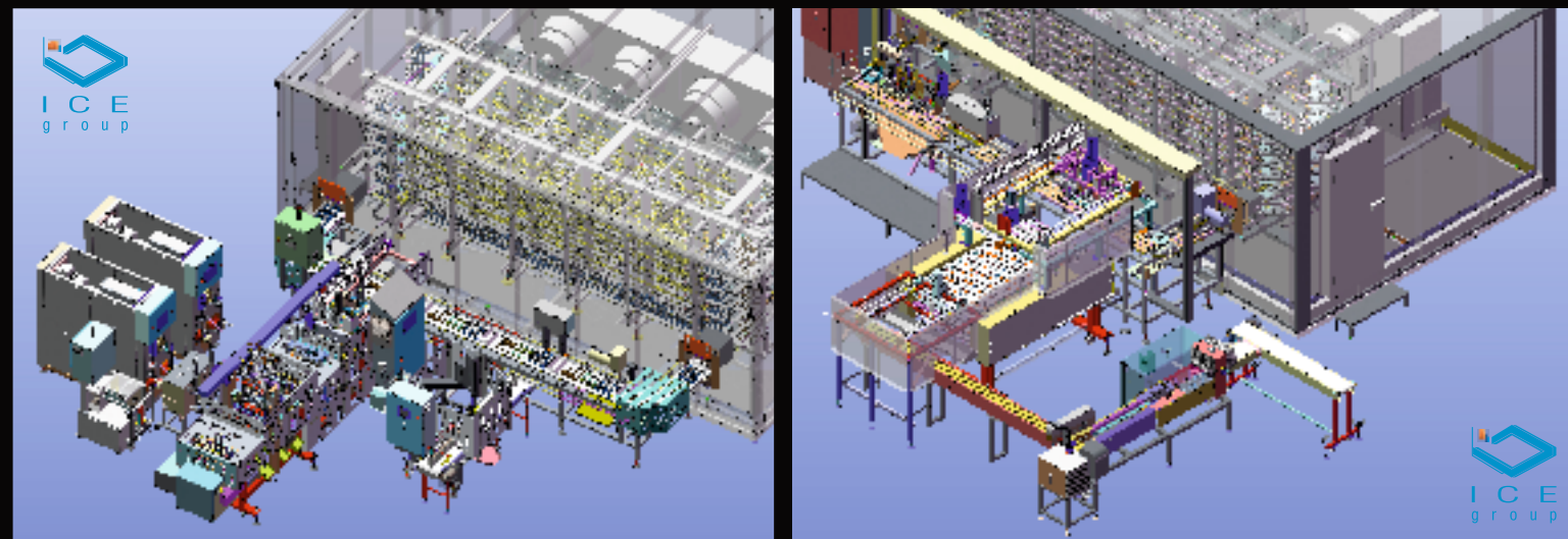
Iglo Line COMPACT 12 000 ▲ with Expert LVF and Jumbo Robot
