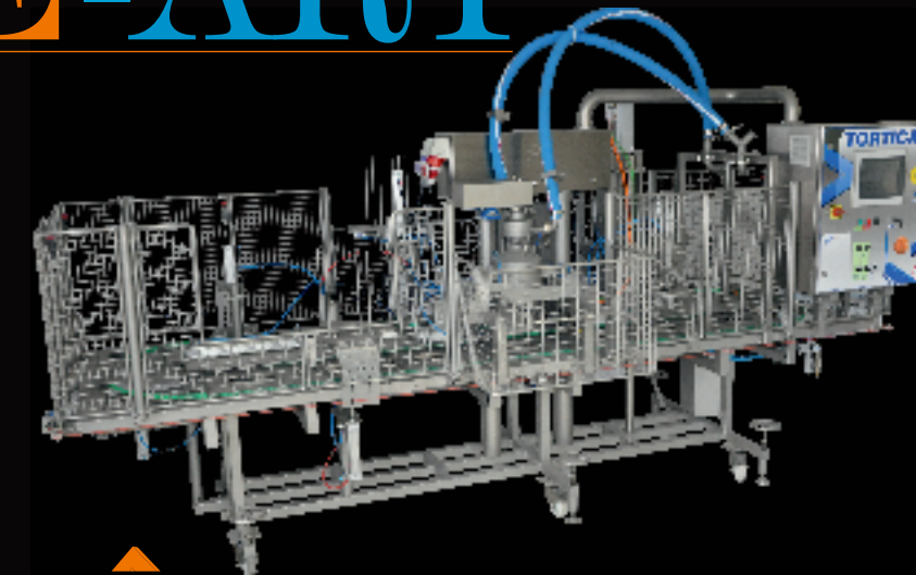
▲ TORTICA MULTI-STATION CAKES AND BULKS FILLER
