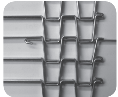
DURAFLEX® Kwik Connect Splice Rod
