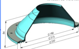
PIPETITE 4" to 6" 10 Holes PCD Ø213 mm
