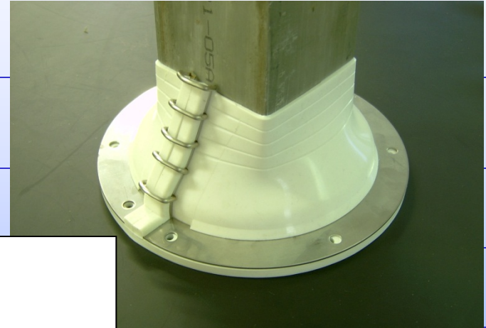
ReBoot on Square Section
