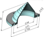
PIPETITE 1/2" to 2-1/2" 4 Holes PCD Ø91 mm
