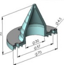
PIPETITE 1/2" to 1 1/4" 4 Holes PCD Ø57 mm
