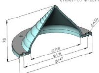
PIPETITE 1/2" to 3" 6 Holes PCD Ø128 mm
