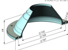
PIPETITE 3" to 5" 8 Holes PCD Ø168 mm
