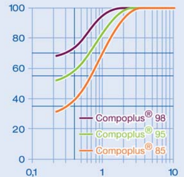
Minimum efficiencies of Compoplus® filter media according to EN779:2012
